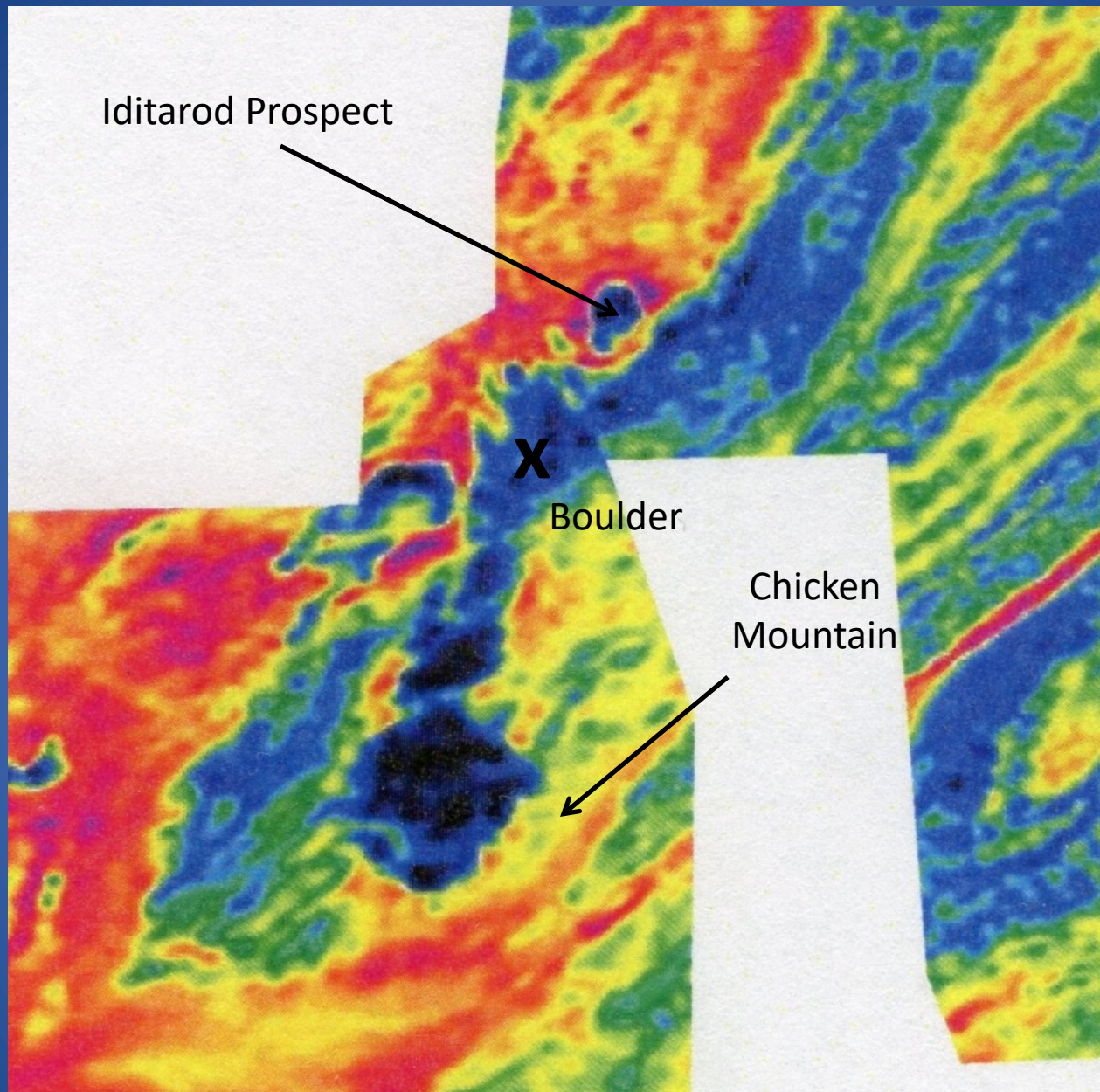
7200 Hz EM showing plutons and volcanic rocks as Resistive
